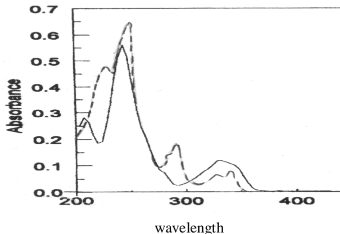
Fig:1 UV absorption spectra of alfuzosin-HCl, 5 µg/ml in water (—) and carvedilol, 5 µg/ml in methanol (---).
