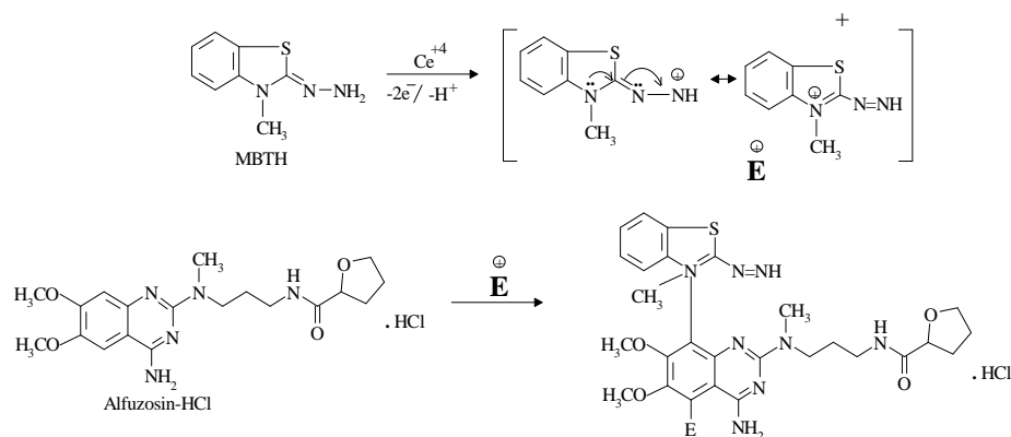
Scheme (1): Proposed Mechanism of the reaction between Alfuzosin-HCl and MBTH/Ce 4+ in acid medium.
